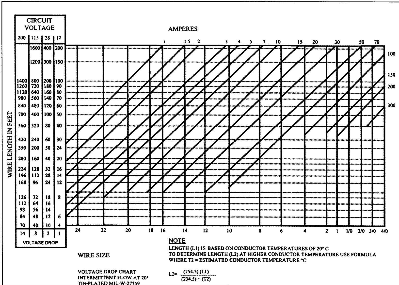
FIGURE 11-3. Conductor chart, intermittent flow.
