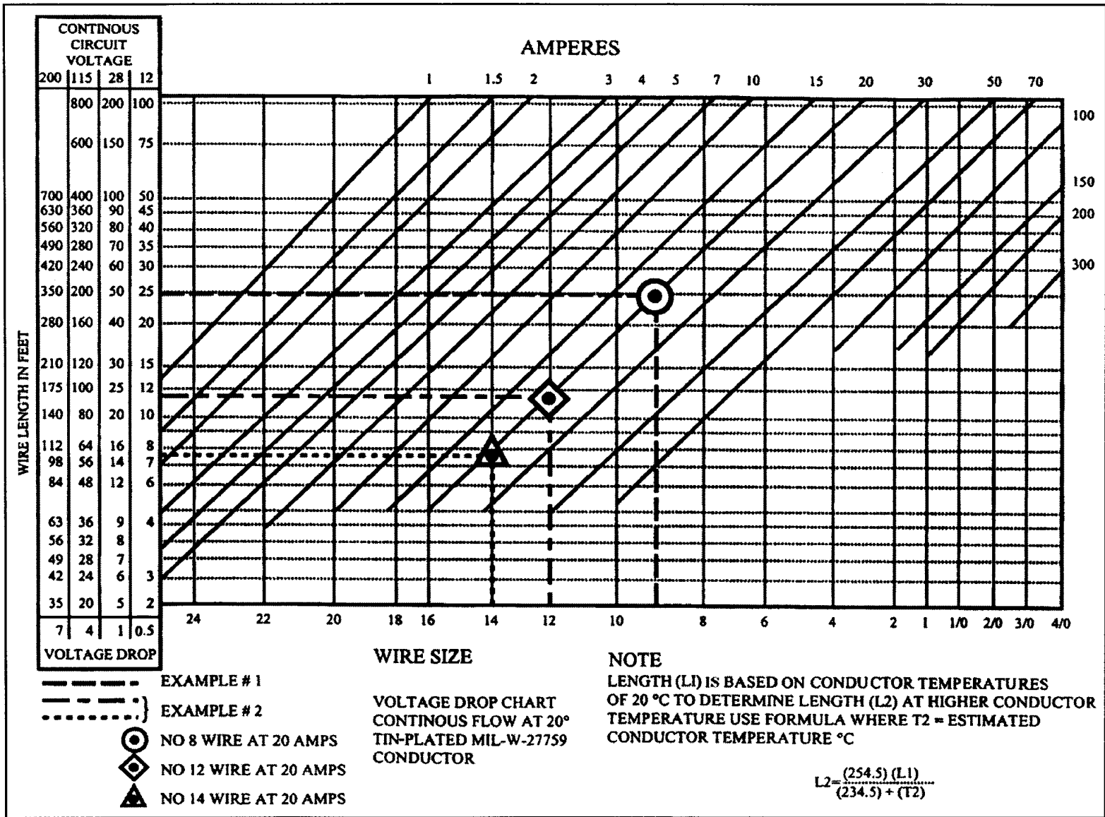
FIGURE 11-2. Conductor chart, continuous flow.
