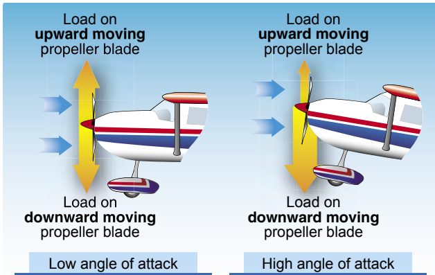
Figure 4-43. Asymmetrical loading of propeller (P-factor).
