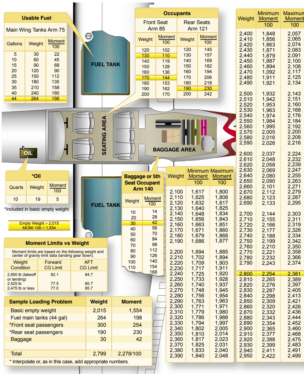
Figure 9-9. Loading schedule placard.
