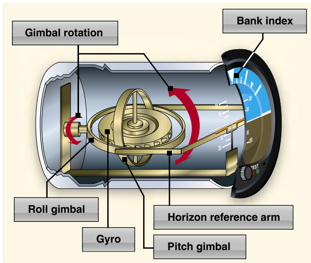
Figure 7-23. Attitude indicator.
