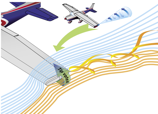
Figure 3-9. Tip vortex.
