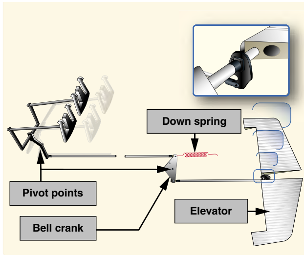
Figure 5-12. When the aerodynamic efficiency of the horizontal tail surface is inadequate due to an aft CG condition, an elevator down spring may be used to supply a mechanical load to lower the nose.
