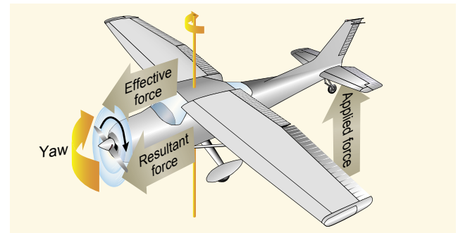
Figure 4-42. Raising tail produces gyroscopic precession.
