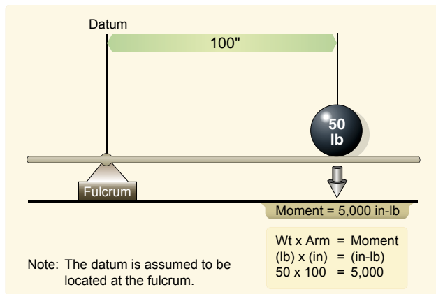
Figure 9-3. Determining moment.
