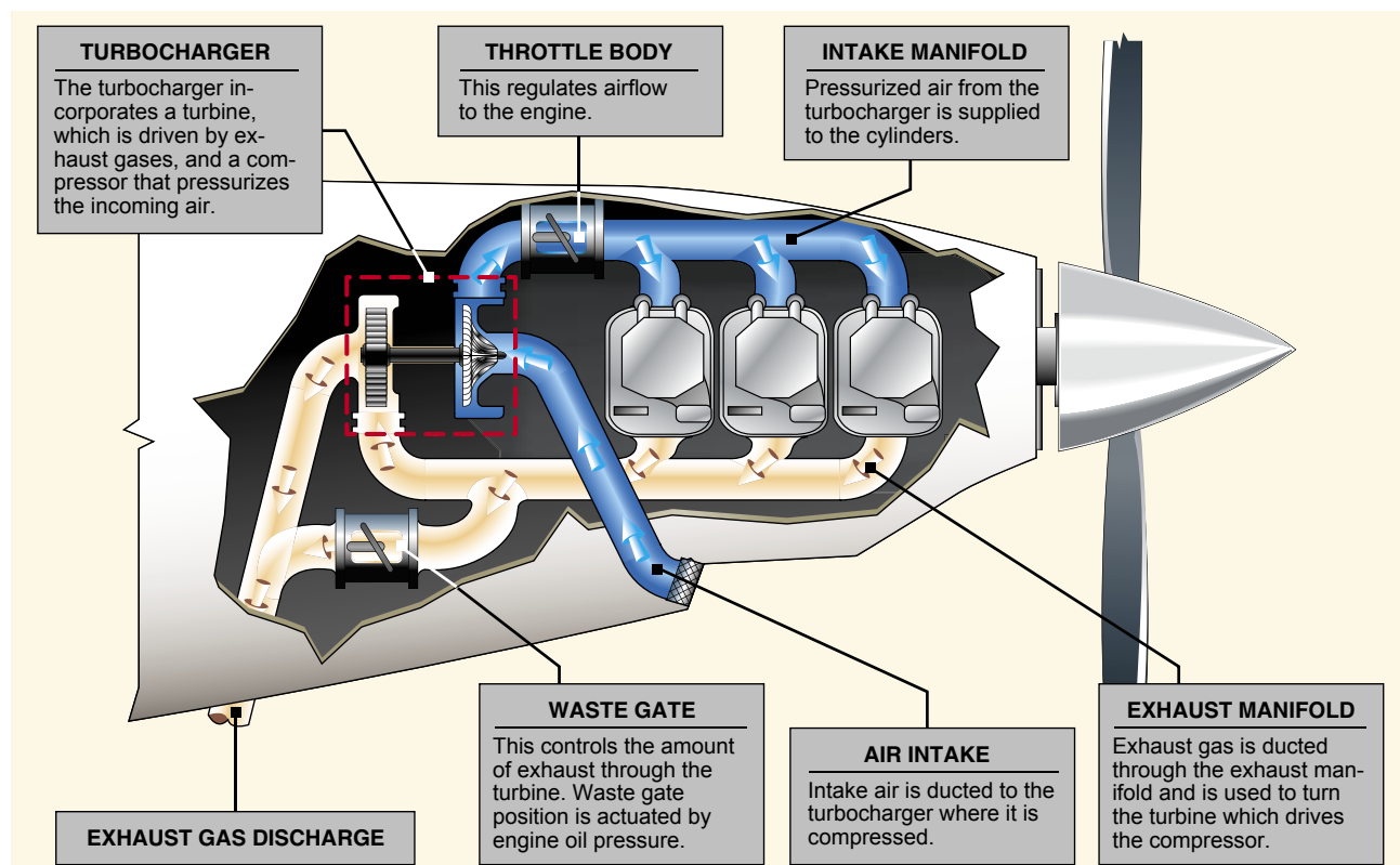
Figure 6-15. Turbocharger components.
