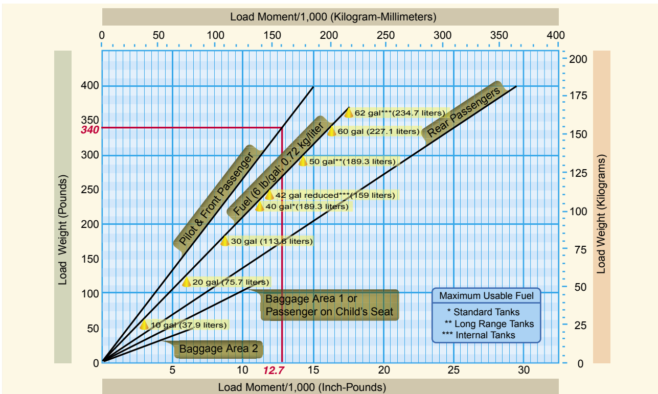
Figure 9-7. Loading graph.
