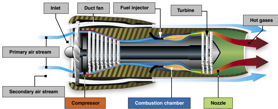
Figure 6-25. Turbofan engine.
