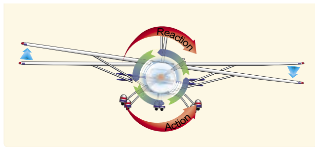
Figure 4-39. Torque reaction.
