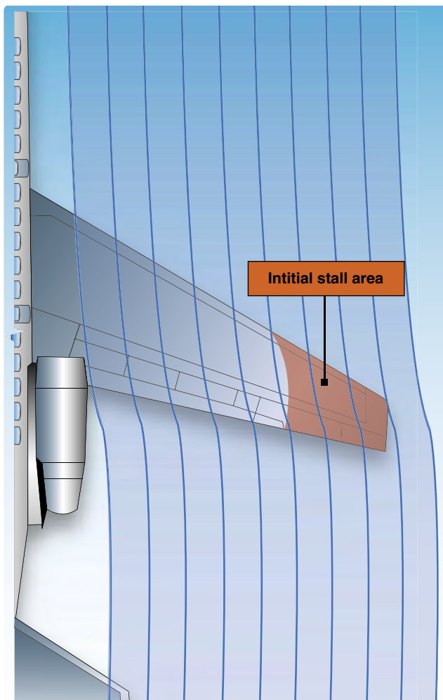
Figure 4-61. Wingtip stall.
