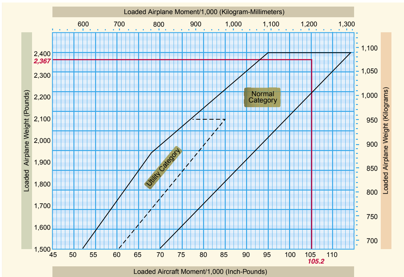
Figure 9-8. CG moment envelope.
