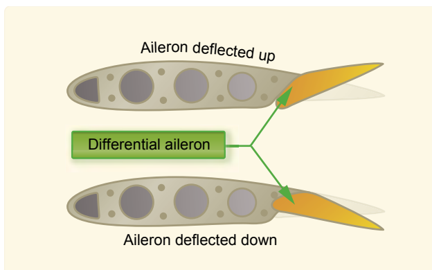
Figure 5-6. Differential ailerons.
